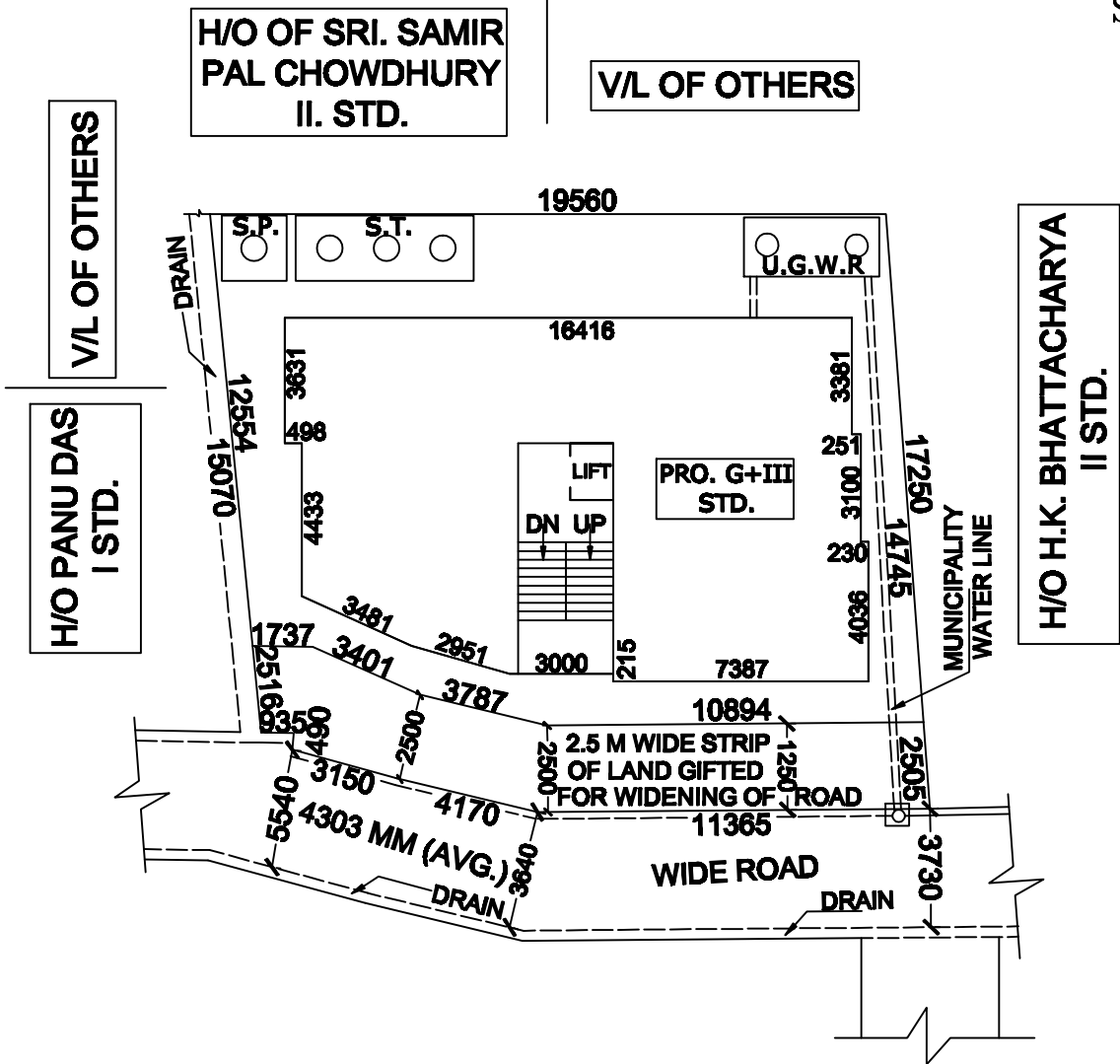
WATER LINE LAYOUT PLAN SCALE = 1:100
